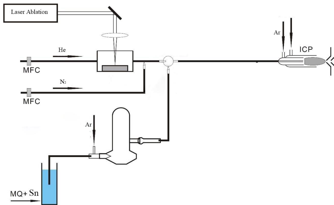
Fig. S1 Schematic diagram of the gas delivery system
