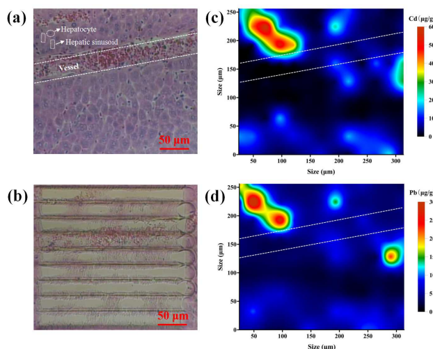
Fig. 5 Quantitative imaging of Pb and Cd in rat liver tissue. (a) microscopic picture of liver tissue before LA analysis; (b) microscopic picture of liver tissue after LA analysis; (c) Cd quantitative imaging; (d) Pb quantitative imaging.
