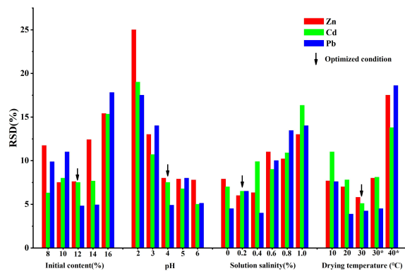
Fig. 3 Relative standard deviation (RSD) of elemental signal in gelatin gels by LA line scanning under different parameters: initial content, pH, solution salinity and temperature. Note: temperature of 10, 20, 30 °C for drying in the oven; 30*, 40* °C for drying at room temperature.
