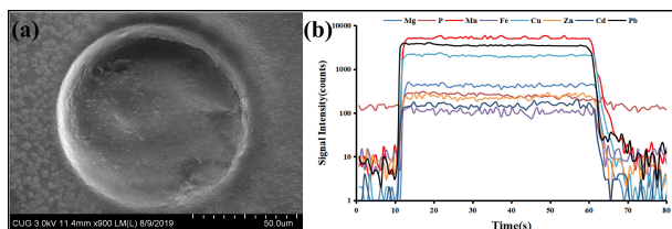
Fig. 4 Ablation crater of gelatin (a) and the signal of the elements (b).
