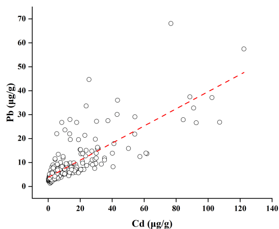
Fig. 6 Correlation between the Cd content and the Pb content in rat liver tissue.
