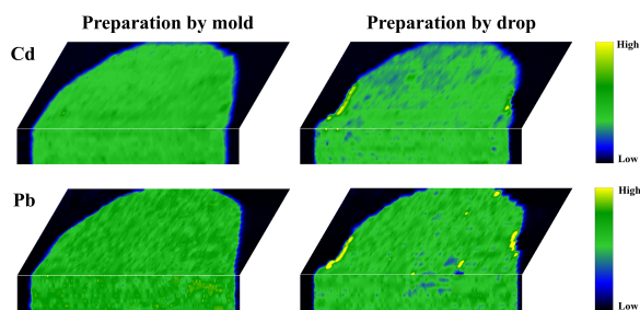
Fig. 2 Spatial distribution of Cd and Pb with and without mold-preparation.
